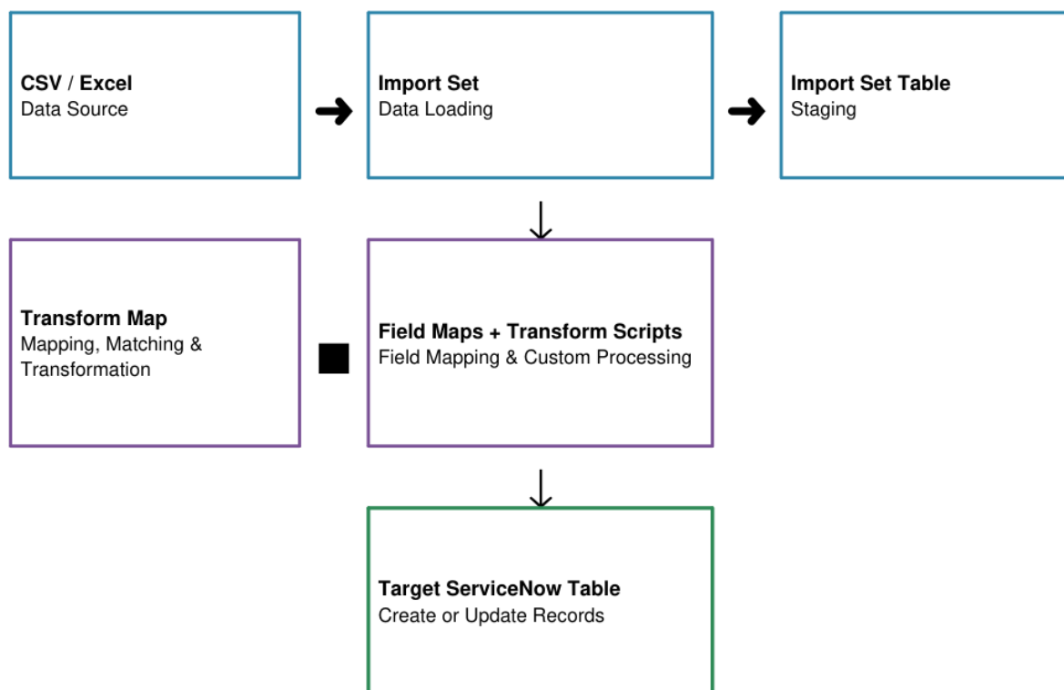
Figure 1: Data flow for importing external data using Transform Maps
